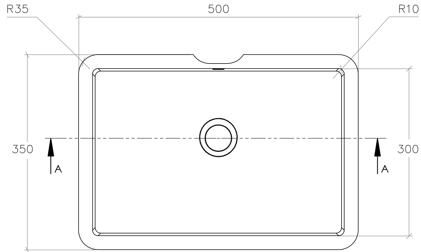
TOP VIEW
